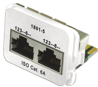
AMP CO Plus Insert, 2-port RJ45 outlet jack, category 6A ethernet, 10/100, white
